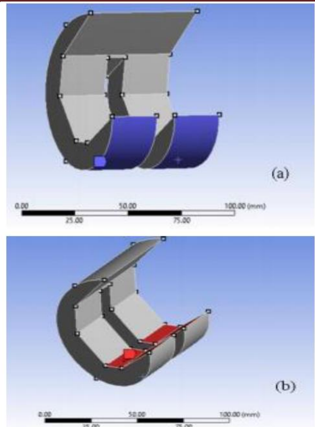
Fig.4 The loading and boundary condition was applied in ANSYS 17 as shown in figure 4 (a) & (b).The load was applied axially in the standing position of knee and it varies from 600 N to 4000 N. The load is applied at femur component by considering the weight of a person.
