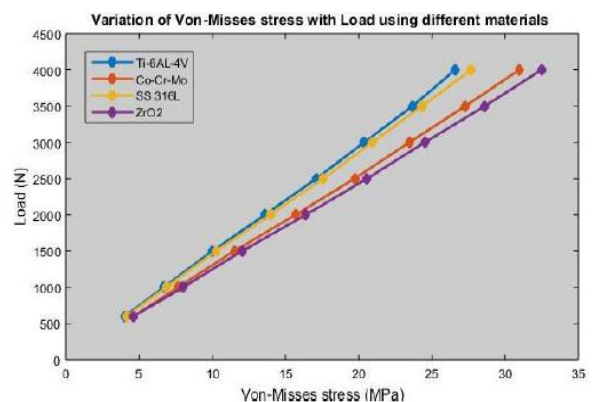
Fig.6: Variation for von-misses stress with load
