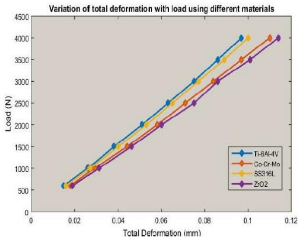
Fig.7: Variation of total deformation with load
