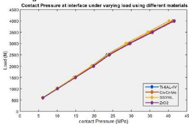
Fig.8: Variation of Contact pressure with load
